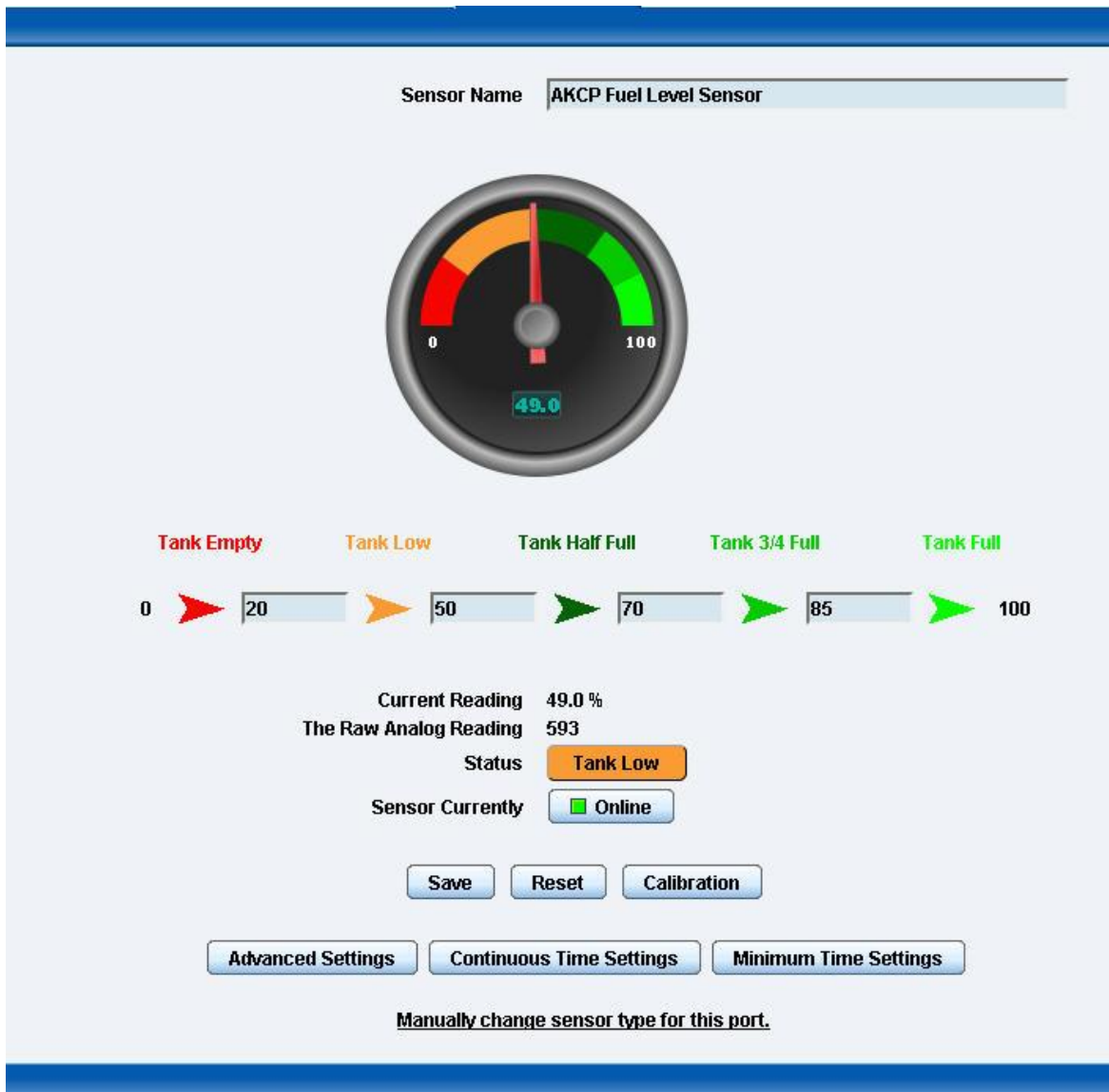
Actual screen shot of the web interface of the fuelLevel Sensor
